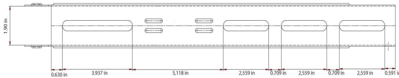
Arm Slot Detail
