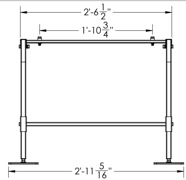
END VIEW RETRACTED
