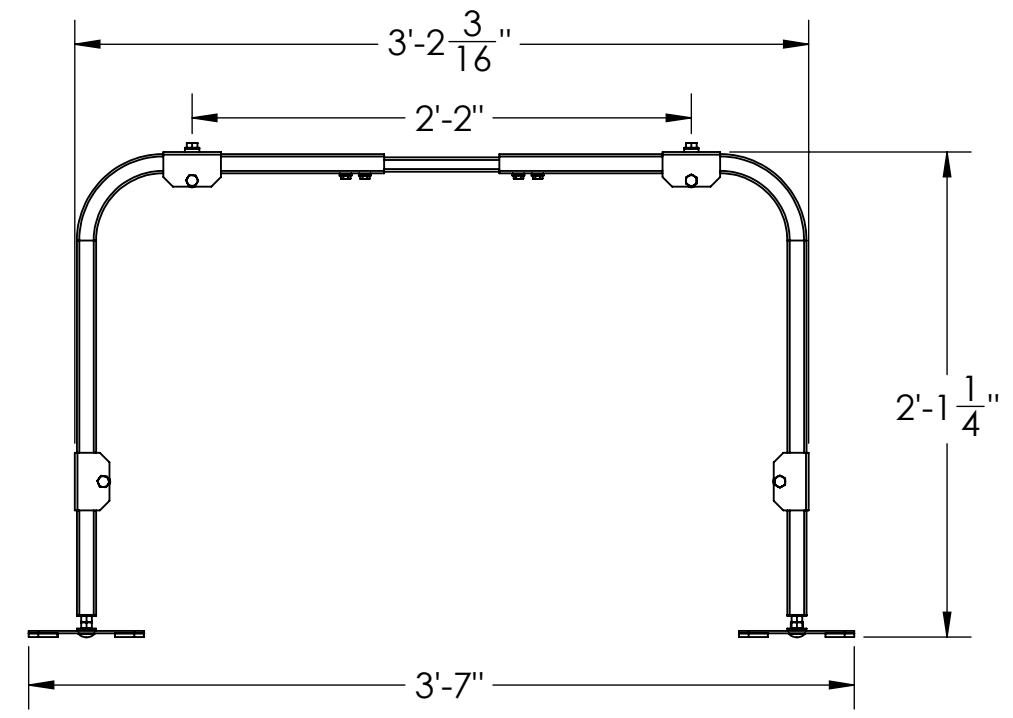
SIDE VIEW EXPANDED
