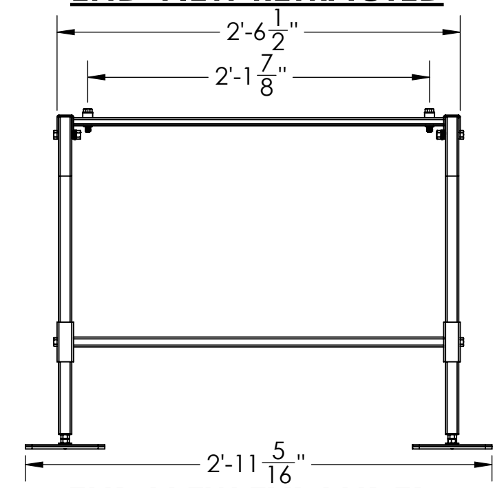
END VIEW EXPANDED
