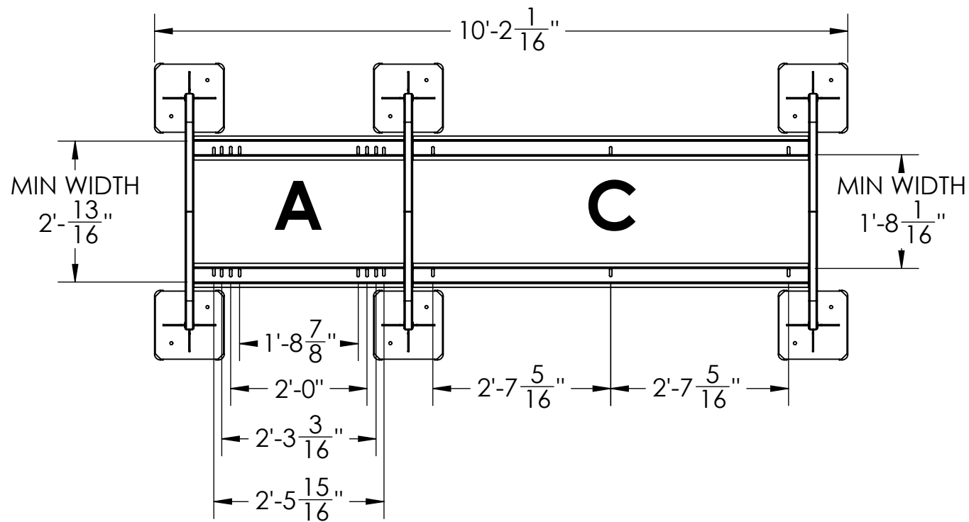
PLAN VIEW RETRACTED
